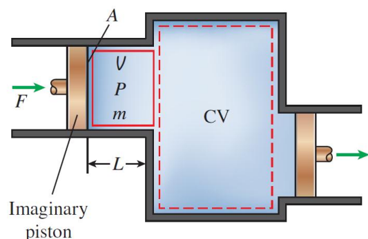
Fig.1.20 – Flow work
