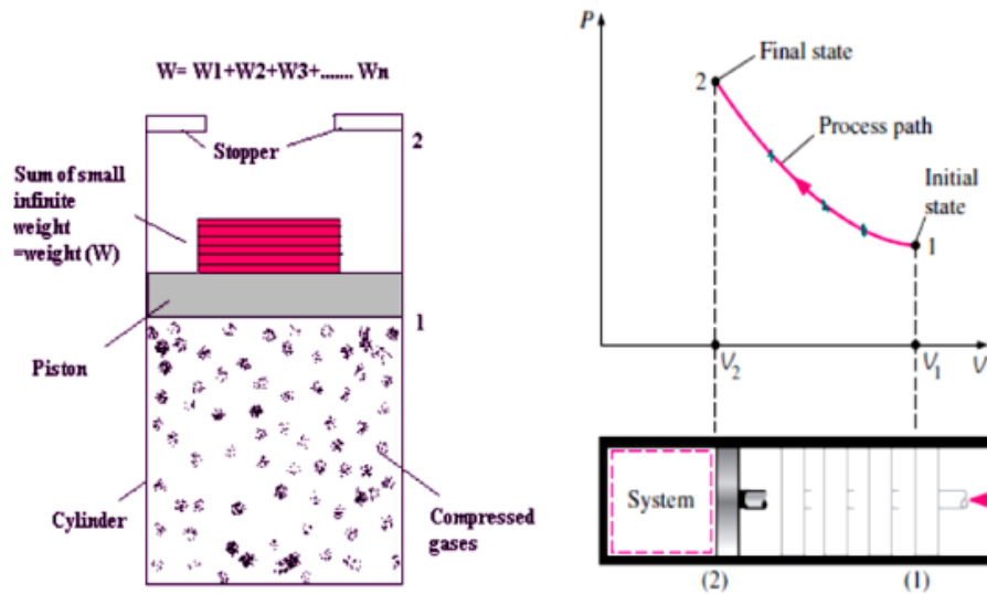
Fig.1.13 – Quasi-static process with p-v diagram of the compression process
