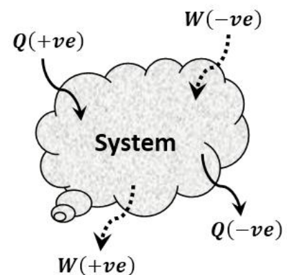
Fig.1.18 – Sign convention for heat and work
