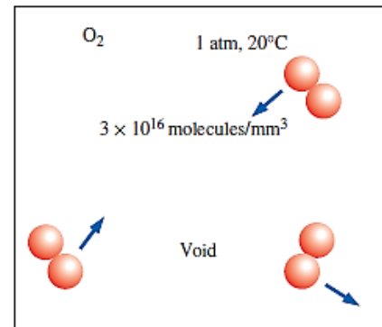
Fig.1.12 – Atoms in Gas Phase
