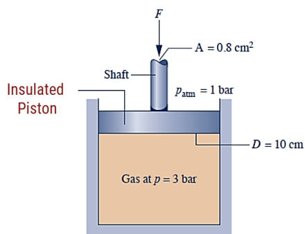
Fig.1.6 – An Adiabatic System
