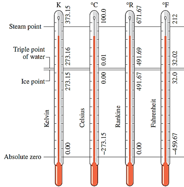
Fig.1.15 – Temperature Scales
