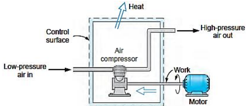
Fig.1.7 – An example of a control volume
