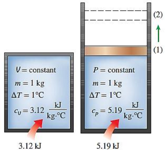
Fig.1.17 – Specific heat at constant volume and constant pressure
