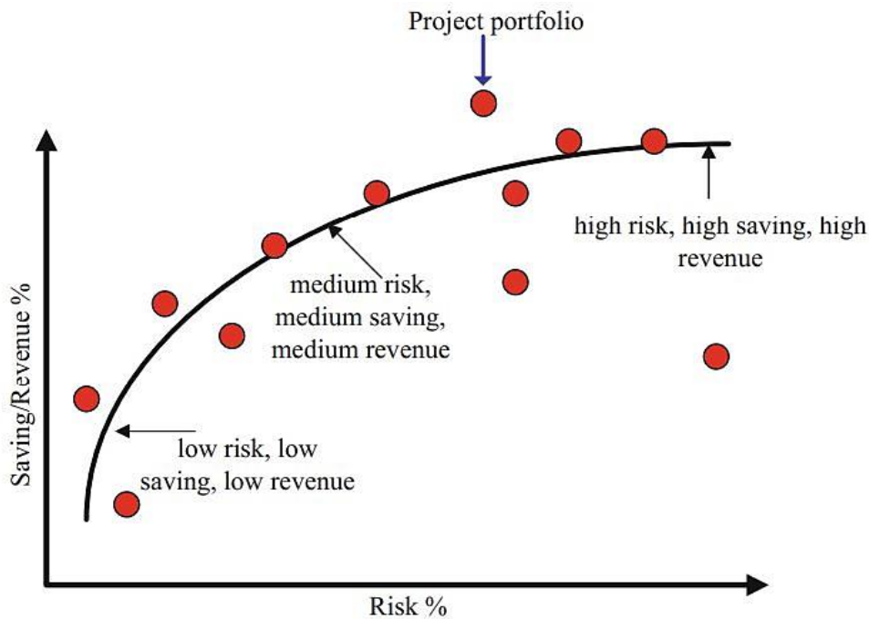
Fig.3.3 – Efficient frontier curve for portfolio selection
